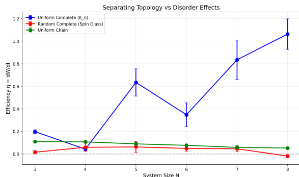
FIG. 4. Disorder vs Topology Effects on Efficiency. Three models isolate disorder and topology effects over N = 3 –8 qubits. Uniform Complete (blue, polynomial DLA) exhibits increasing efficiency with system size ( \eta \approx 0.2 \rightarrow 1.0 ), demonstrating “constructive scaling” where all-to-all connectivity provides additional information pathways. Uniform Chain (green, polynomial DLA) maintains small positive efficiency ( \eta \approx 0.05 –0.1), limited by connectivity but stable. Random Complete (red, exponential DLA) collapses to \eta < 0 at N \geq 8 , confirming that coupling disorder (frustration)—not graph topology—drives the exponential DLA growth and thermodynamic crash.
