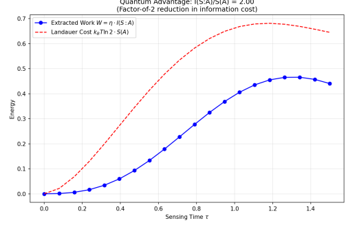
FIG. 2. Landauer Analysis of the Quantum Engine. Extracted work (blue) vs. Landauer erasure cost (red dashed) as a function of sensing time \tau . The constant ratio I(S:A)/S(A) = 2.00 is the mathematical signature of pure bipartite entanglement ( I = 2S by definition for pure states), confirming that the feedback mechanism operates via quantum correlations rather than classical correlations (which would yield I \leq S ).
